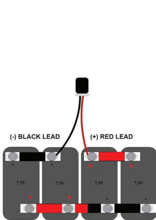
Figure 1: +15 VOLT Standard Battery Configuration Series/Parallel configuration requires two (1) set of 7.5 Volt Batteries (NFES # 1023)
