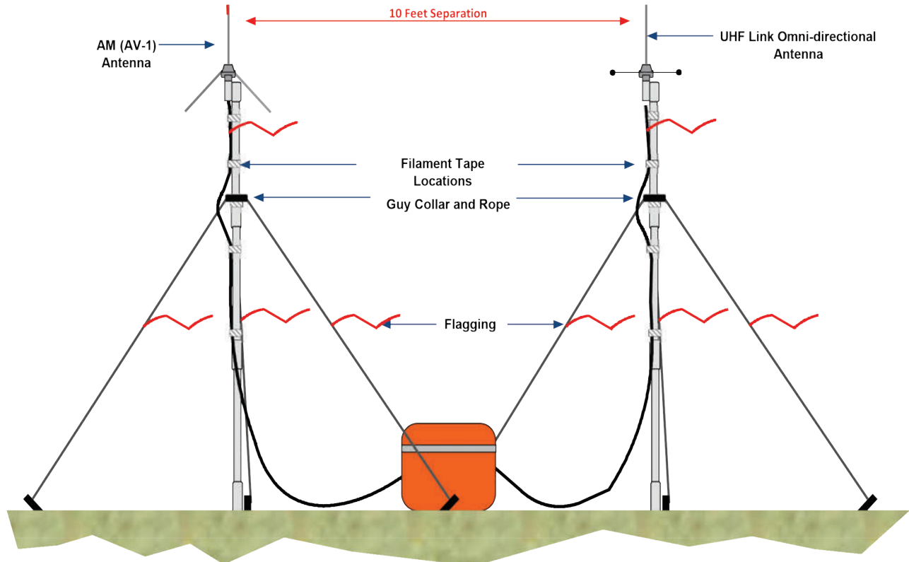
Figure 4: 4370 GROUND AIRCRAFT RADIO/LINK ANTENNA SETUP LINK CONFIGURATION
