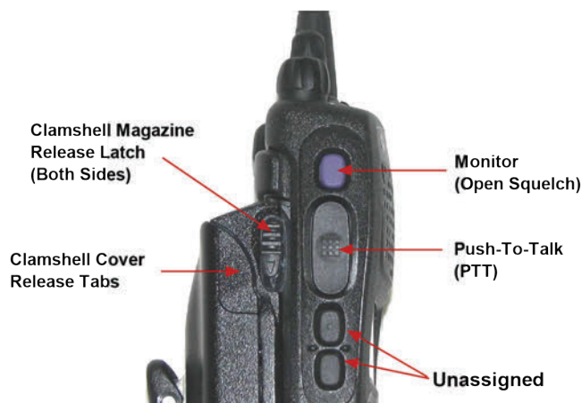
Figure 2: Side View XTS 2500
