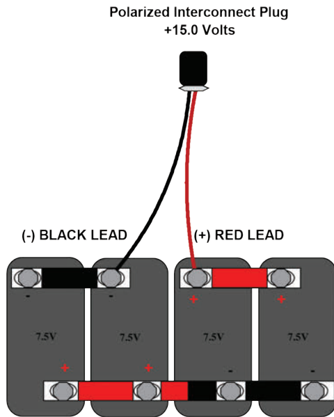
Figure 1: 15 VOLT BATTERY CONFIGURATION (NFES # 1023)
