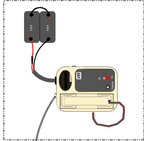
Figure 6: CPI DC Remote Connections Located in COMM Operating on DC Power
