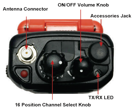
Figure 2: Top View Midland
