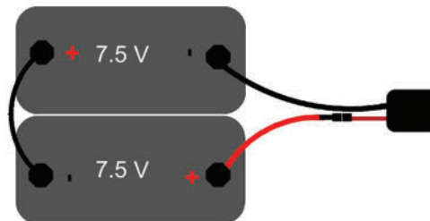
Figure 3: +15 VOLT Series Battery Configuration Series configuration requires two (2) each of 7.5 Volt Batteries
