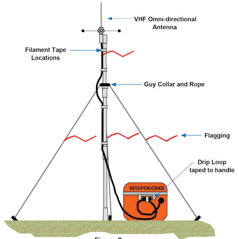
Figure 2: 4312 - VHF REPEATER ANTENNA SETUP STAND-ALONE CONFIGURATION
