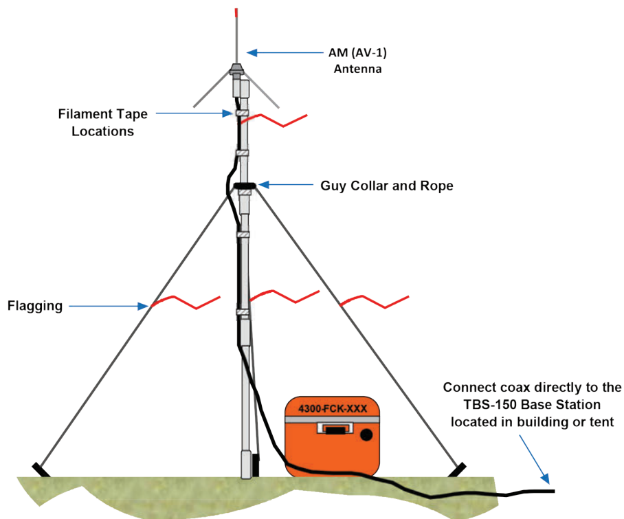
Figure 2: 4300 - GROUND VHF-AM BASE STATION ANTENNA SETUP
