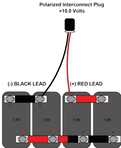
Figure 1: 15 VOLT BATTERY CONFIGURATION (NFES # 1023)
