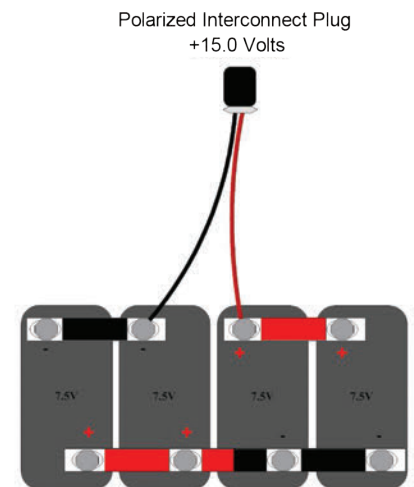
Figure 4: 15 VOLT BATTERY CONFIGURATION (NFES # 1023)
