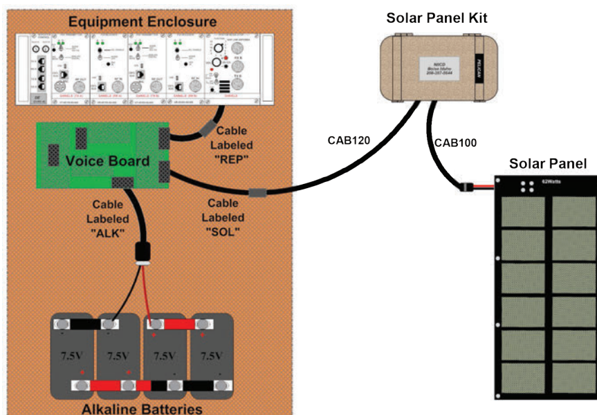
Figure 1: Voice Board Block Diagram Note: Voice Board is physically attached to the back of the equipment.
