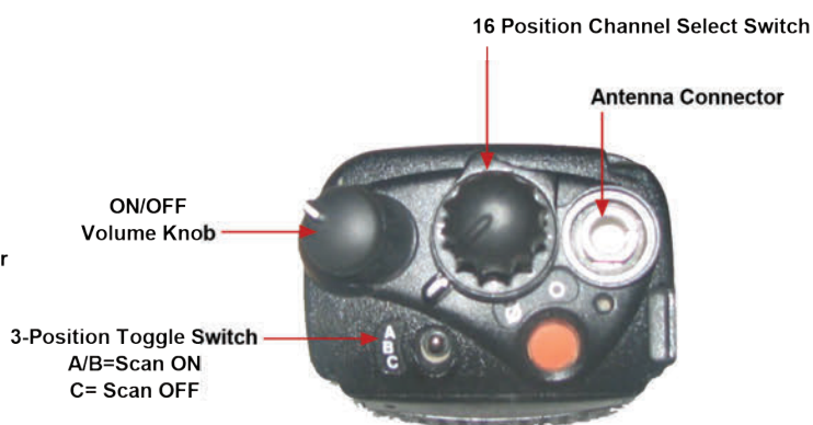
Figure 3: Top View XTS 5000
