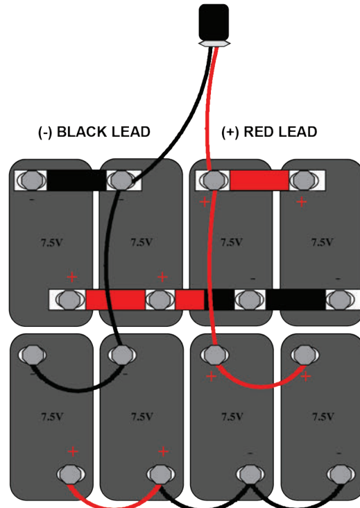
Figure 2: +15 VOLT Double Battery Configuration Series/Parallel configuration requires two (2) sets of 7.5 Volt Batteries (NFES # 1023)
