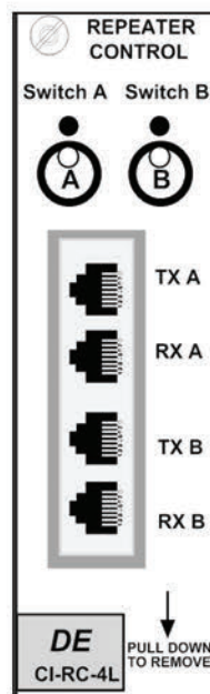
Figure 3: 4312 - VHF COMMAND REPEATER/LINK REPEATER CONTROL MODULE
